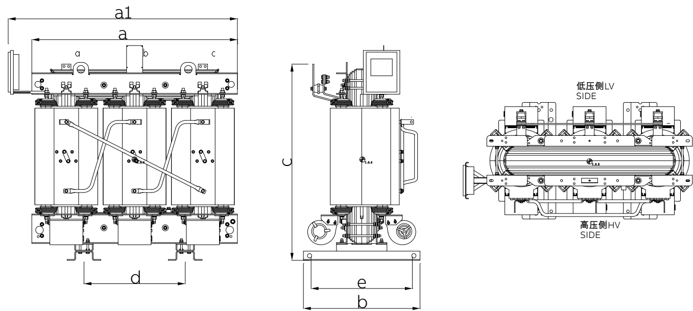
VCC 干式变压器IP00外形图 Outline of VCC with IP00 enclosure
